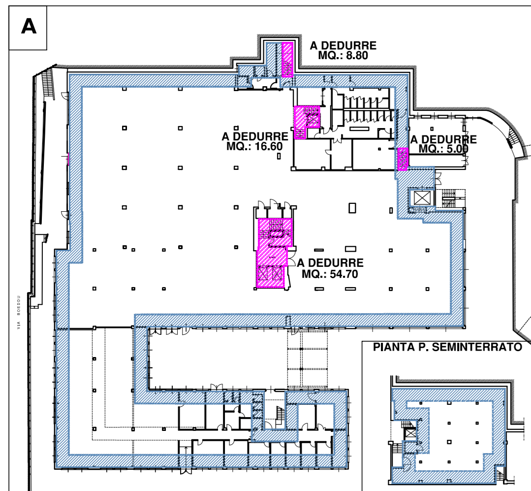
-PIANTA PIANO TERRA E PIANO SEMINTERRATO-
