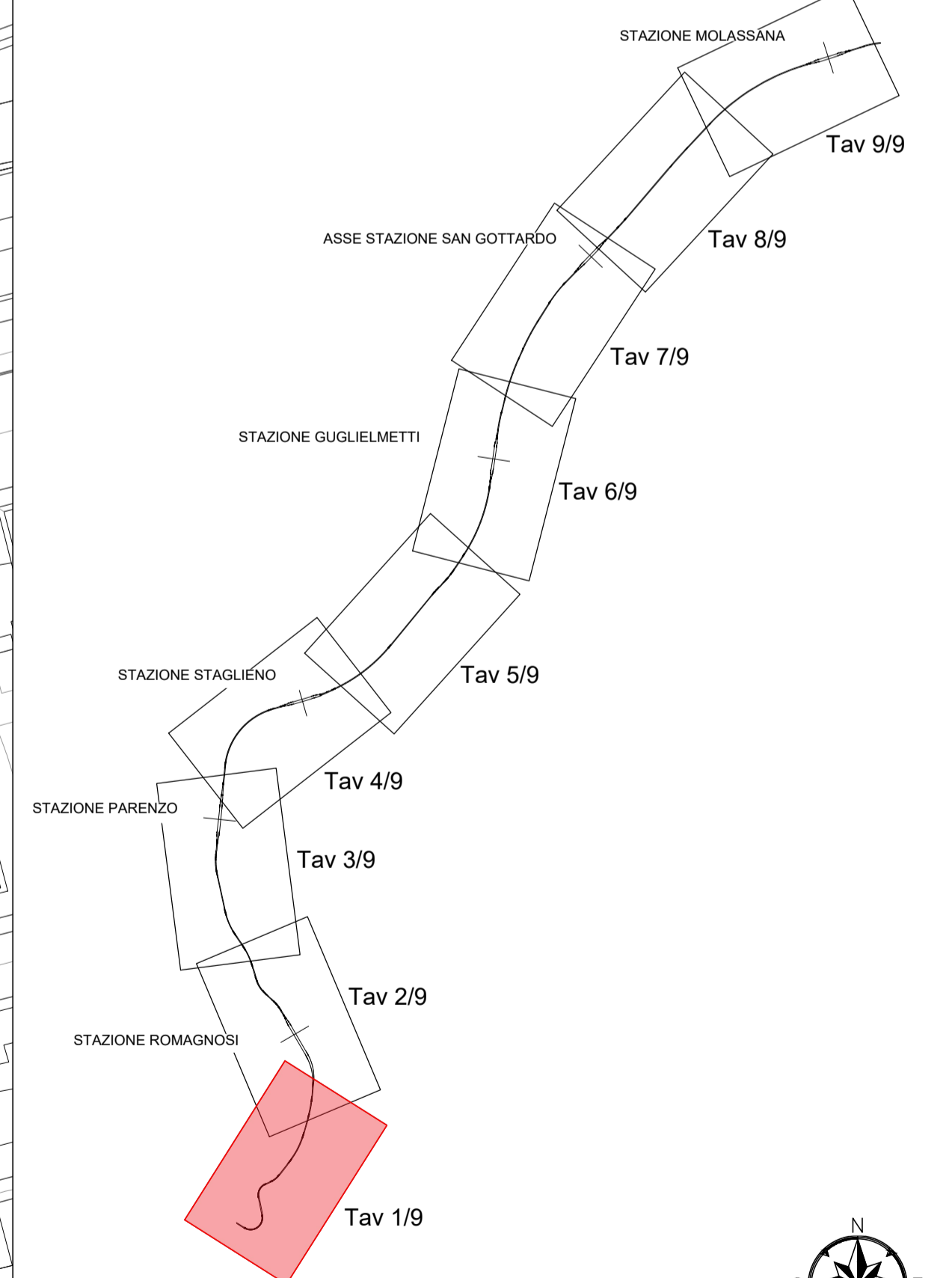
KEY PLAN
