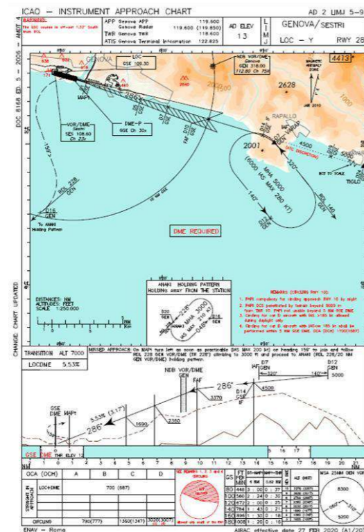
Figura 4.20 LOC-Y RWY28 – AIP ITALIA A1/20
