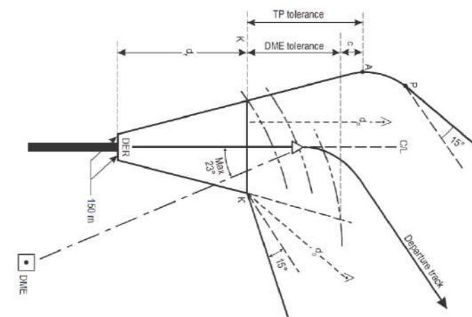
Figura 4.13 ICAO Turning Departure
