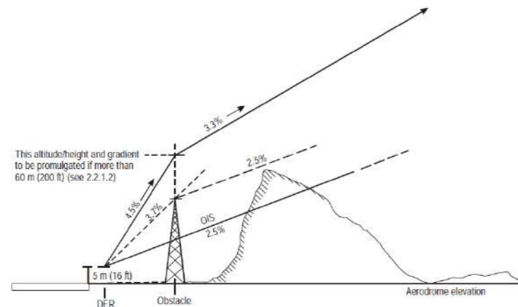
Figura 4.14 ICAO Procedure Design Gradient
